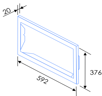
IMI30ST3 Trim Kit dimensions
