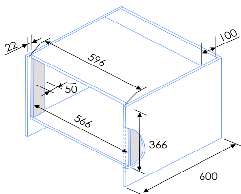
Figure 1 Building - In Cabinet requirements
